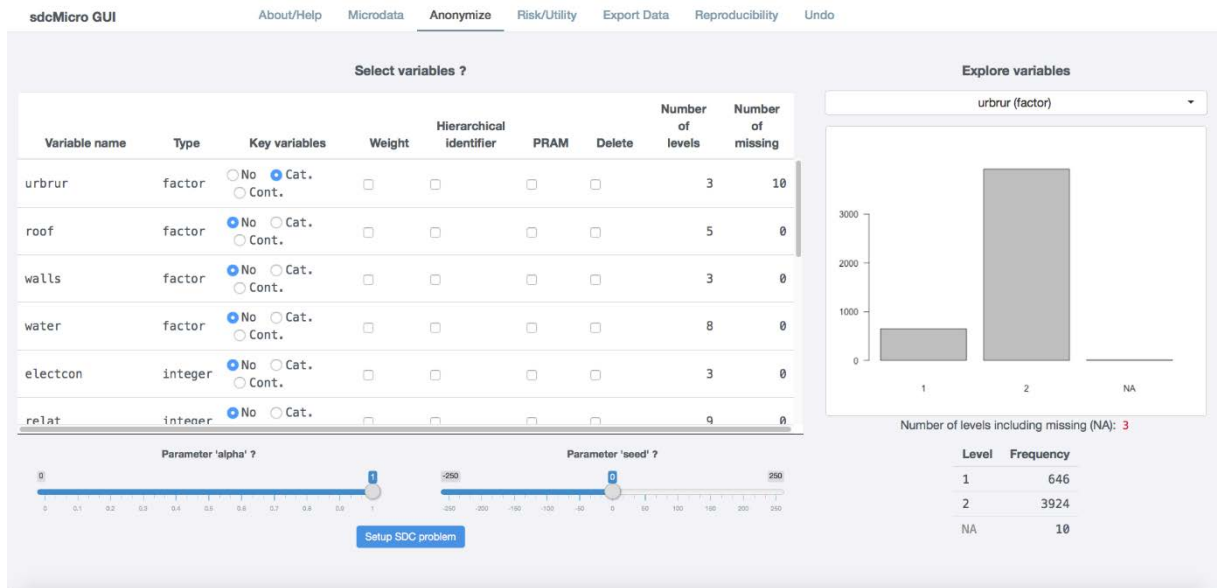
Screenshot 3 Anonymize tab with the interactive variable selection table
